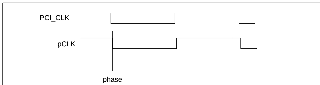
Figure 3-6. Phase Offset in Clock Slave Mode – Frequency > 33 MHz
