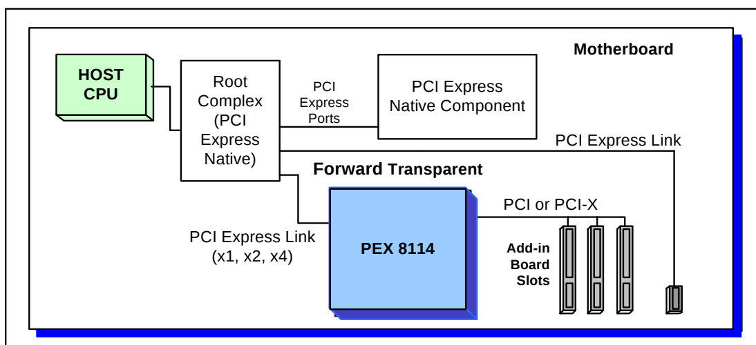
Figure 1-7. PEX 8114 on Motherboard Provides PCI/PCI-X Slots
