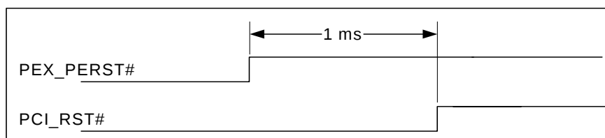
Figure 3-9. PEX_PERST# and PCI_RST# Timing in Reverse Transparent Bridge Mode
