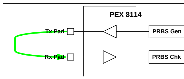
Figure 15-3. Cable Loopback
